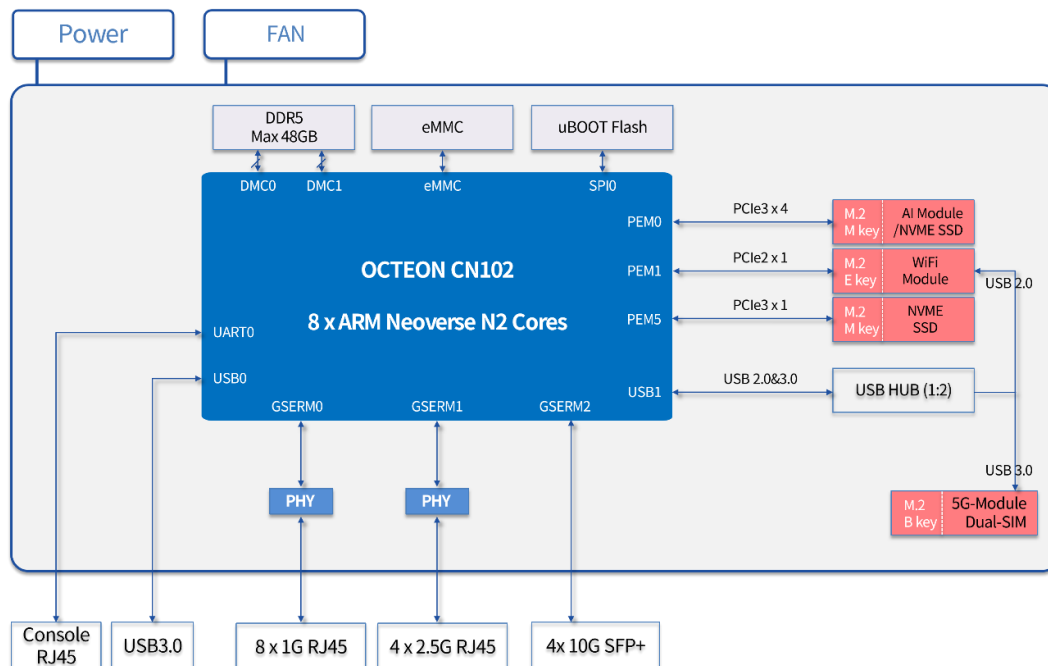
ET2500 Edge Network Appliance system architecture
