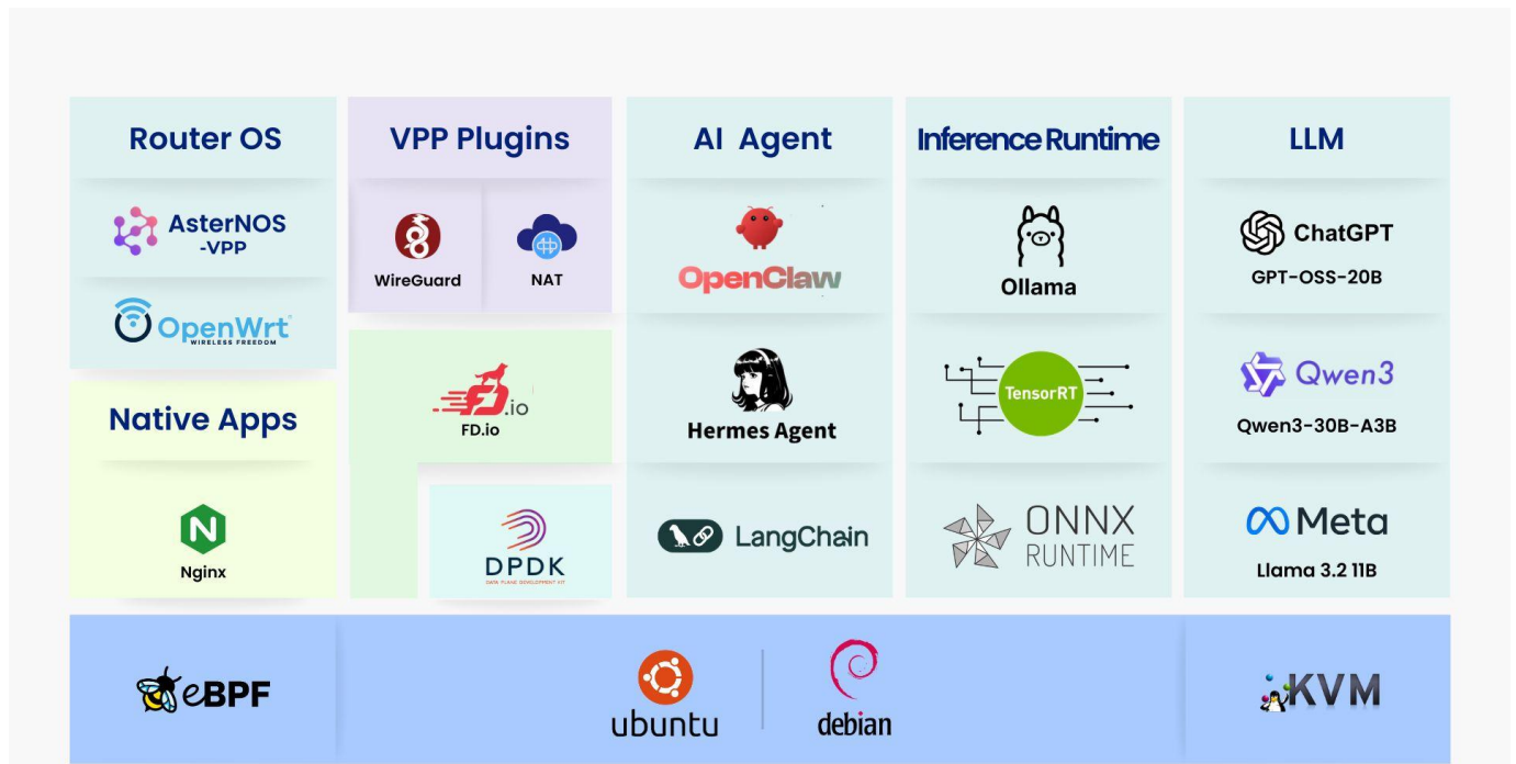
Software Ecosystem
